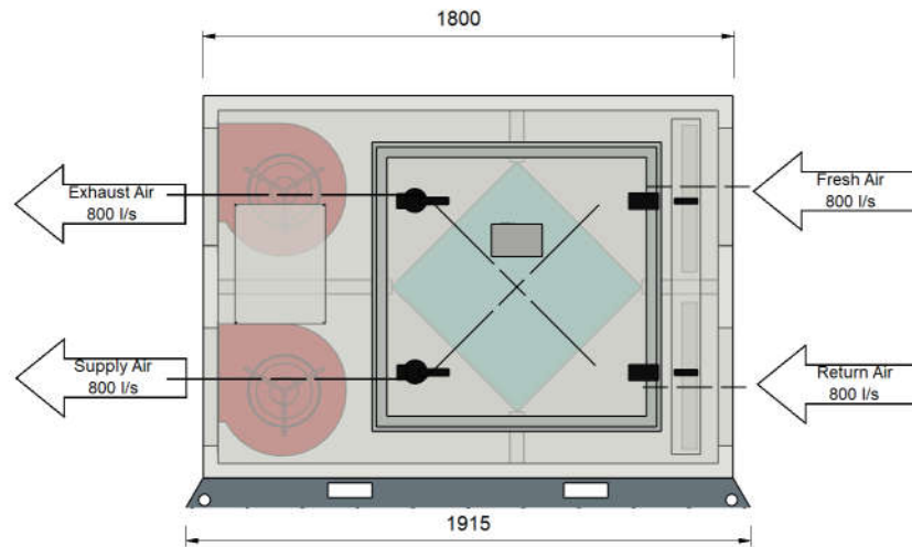
ELEVATION VIEW - ACCESS PANELS SIDE
