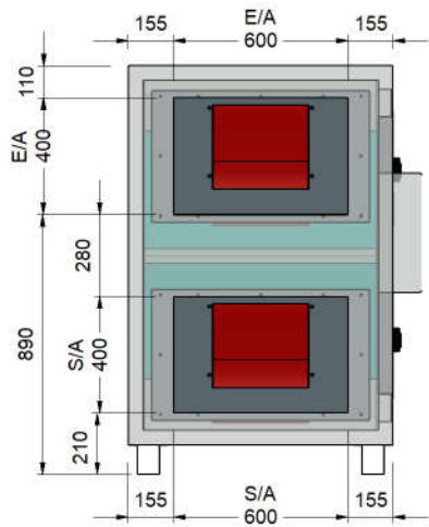
E/A & S/A SPIGOTS
