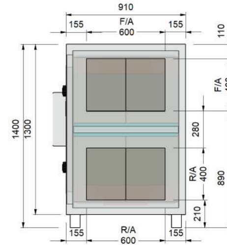
F/A & R/A SPIGOTS
