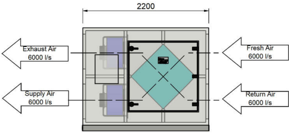
ELEVATION VIEW - ACCESS PANEL SIDE
