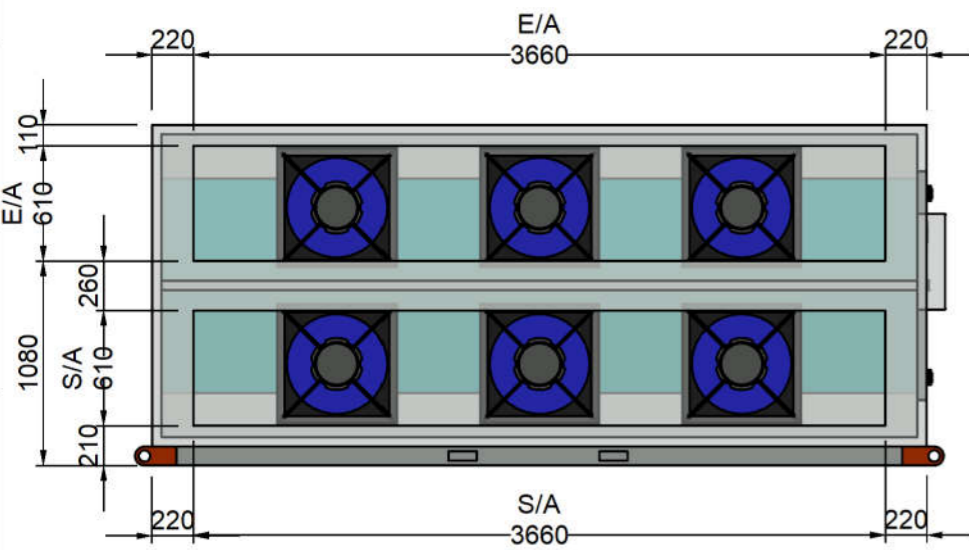
E/A & S/A SPIGOTS
