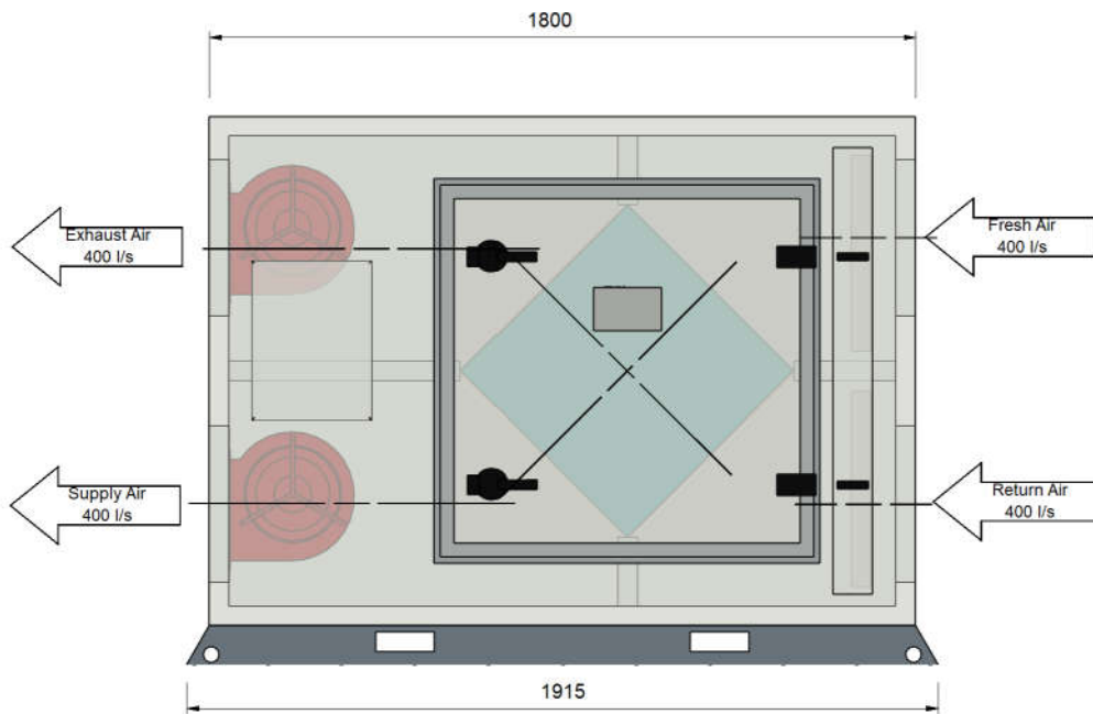
ELEVATION VIEW - ACCESS PANELS SIDE
