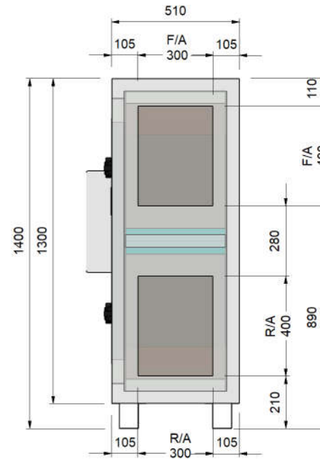
F/A & R/A SPIGOTS
