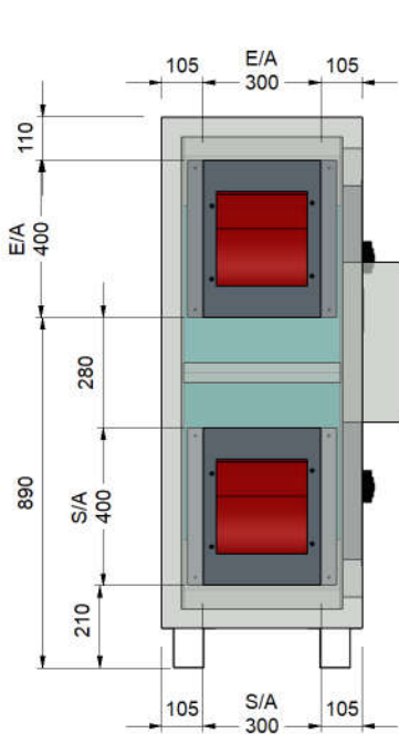
E/A & S/A SPIGOTS
