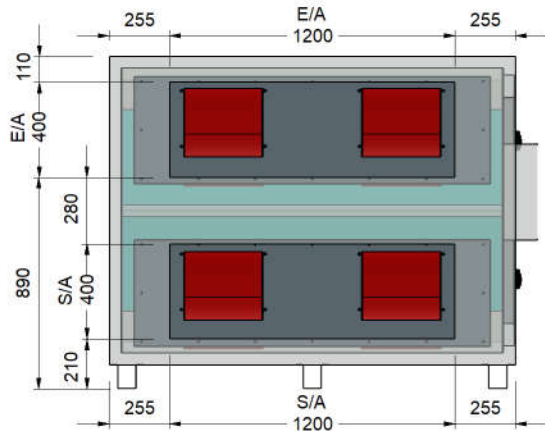
E/A & S/A SPIGOTS
