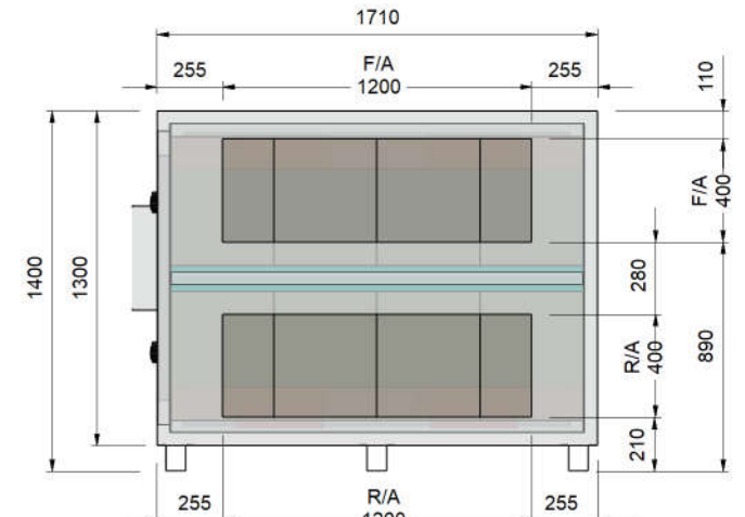
F/A & R/A SPIGOTS
