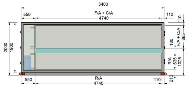
FA & RA SPIGOT VIEW
