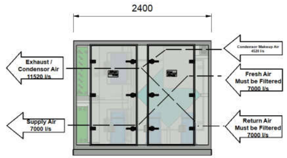
ELEVATION VIEW - COMPRESSOR ACCESS PANEL SIDE
