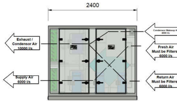
EVAPORATION VIEW - COMPRESSOR ACCESS PANEL SIDE
