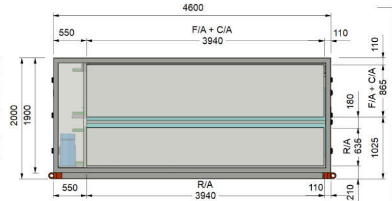
FA & RA SPIGOT VIEW
