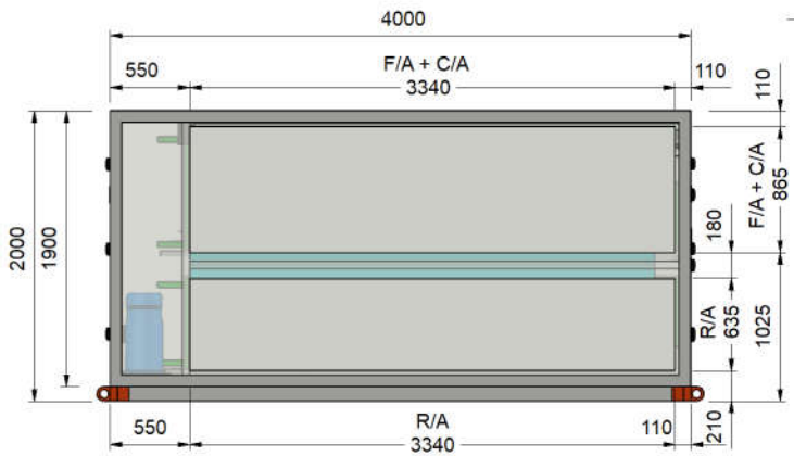
FA & RA SPIGOT VIEW
