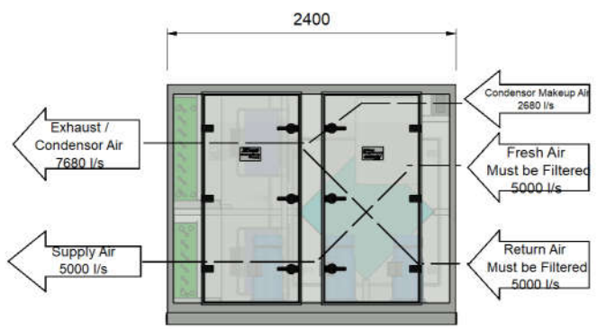
ELEVATION VIEW - COMPRESSOR ACCESS PANEL SIDE
