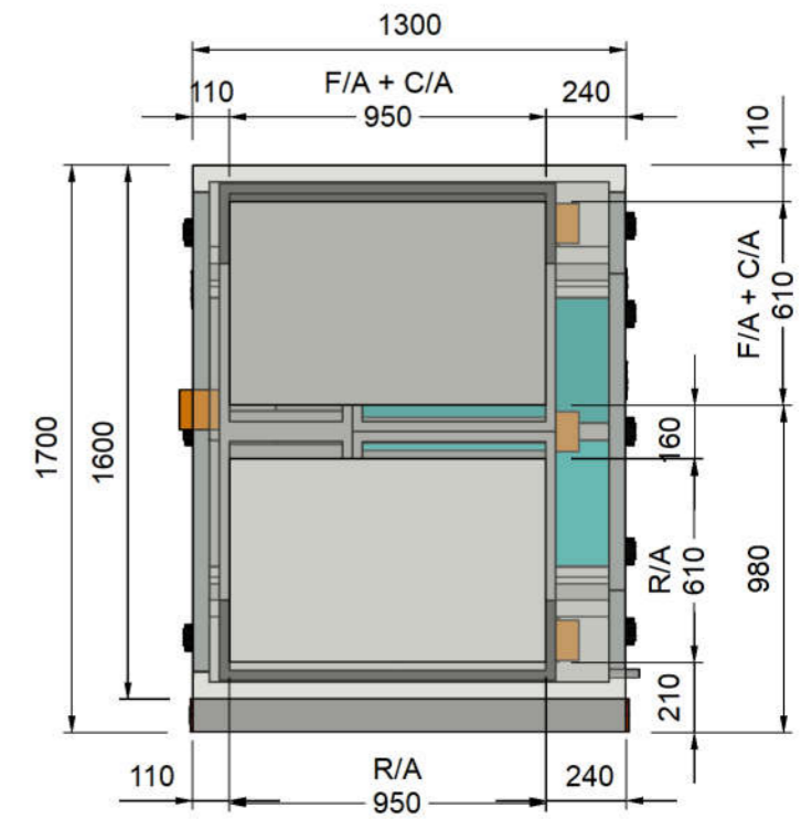
FA & RA SPIGOT VIEW
