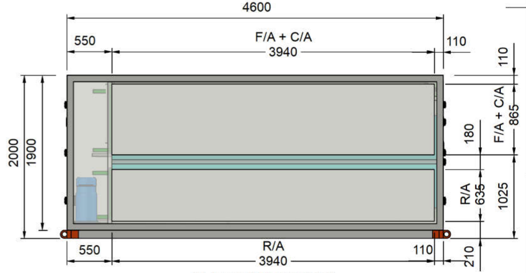
FA & RA SPIGOT VIEW
