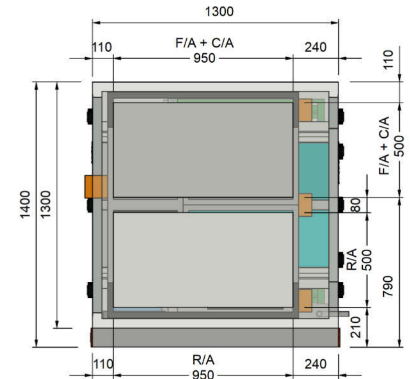
FA & RA SPIGOT VIEW
