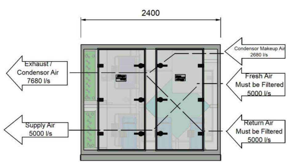
COMPRESSOR A/P PLAN VIEW
