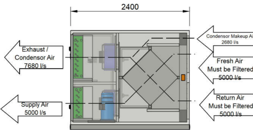
ELEVATION VIEW - FAN ACCESS PANEL SIDE
