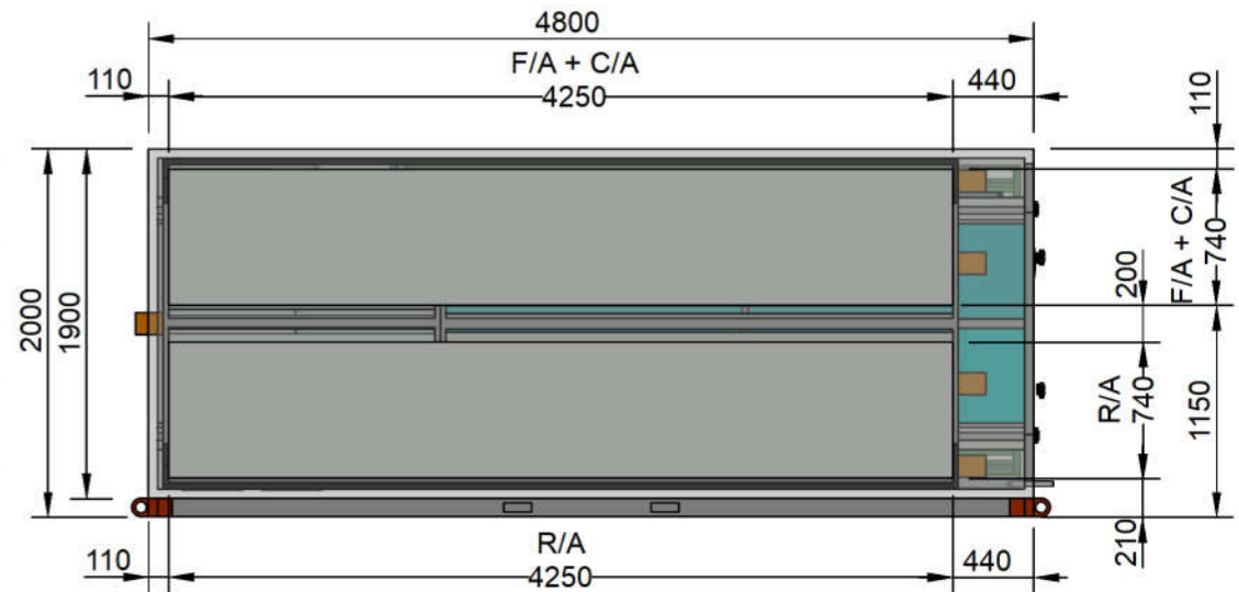
F/A & R/A SPIGOTS
