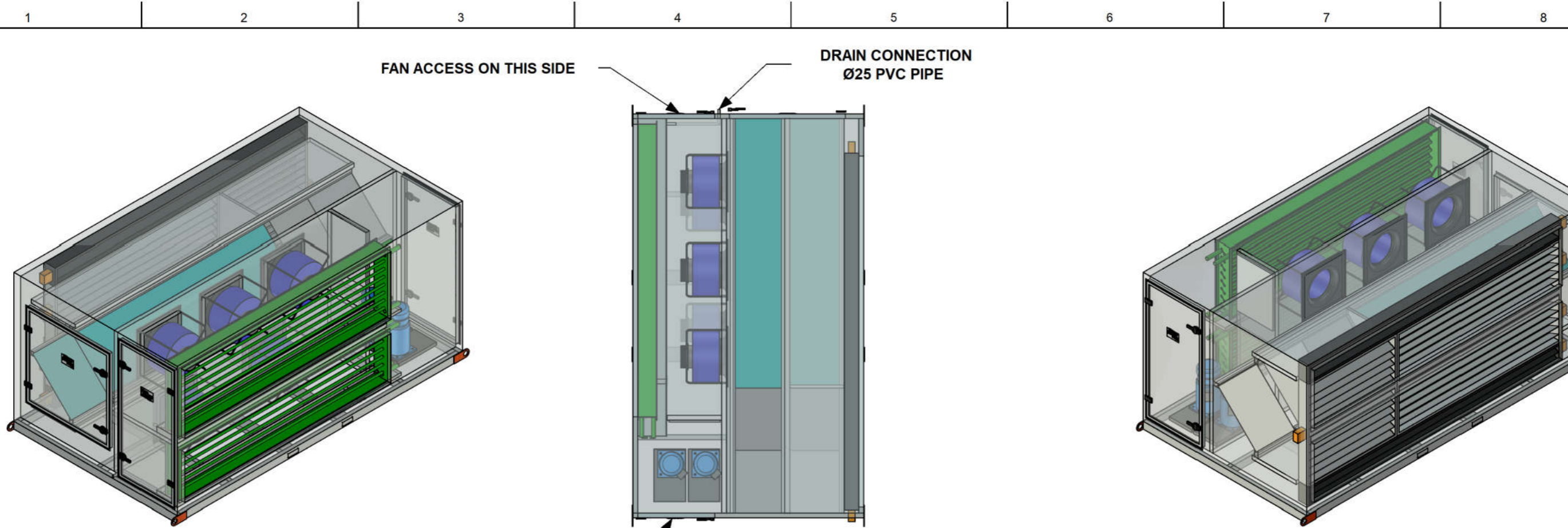
PLAN VIEW
