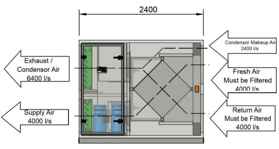
ELEVATION VIEW - MEDIA ACCESS PANEL SIDE
