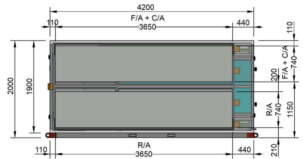
F/A & R/A SPIGOTS
