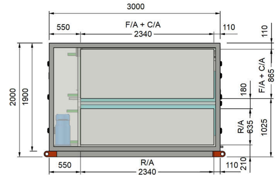
FA & RA SPIGOT VIEW
