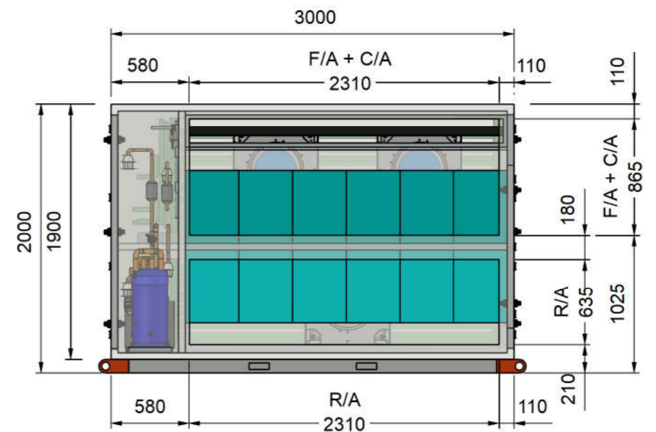
FA & RA SPIGOT VIEW
