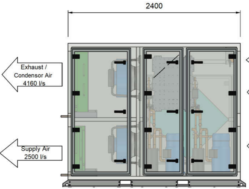
ELEVATION VIEW - ACCESS PANELS SIDE
