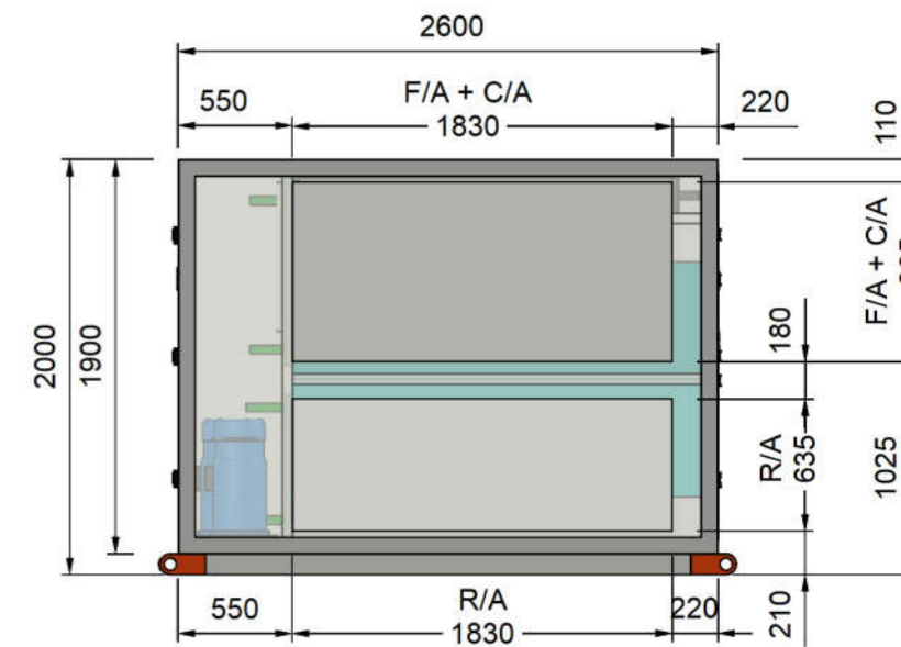
FA & RA SPIGOT VIEW
