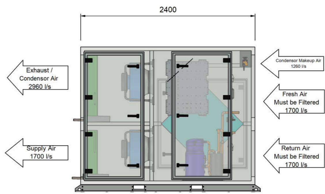
ELEVATION VIEW - ACCESS PANELS SIDE
