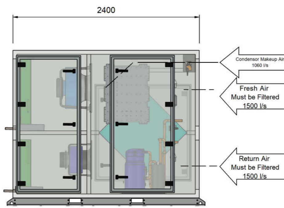
ELEVATION VIEW - ACCESS PANELS SIDE
