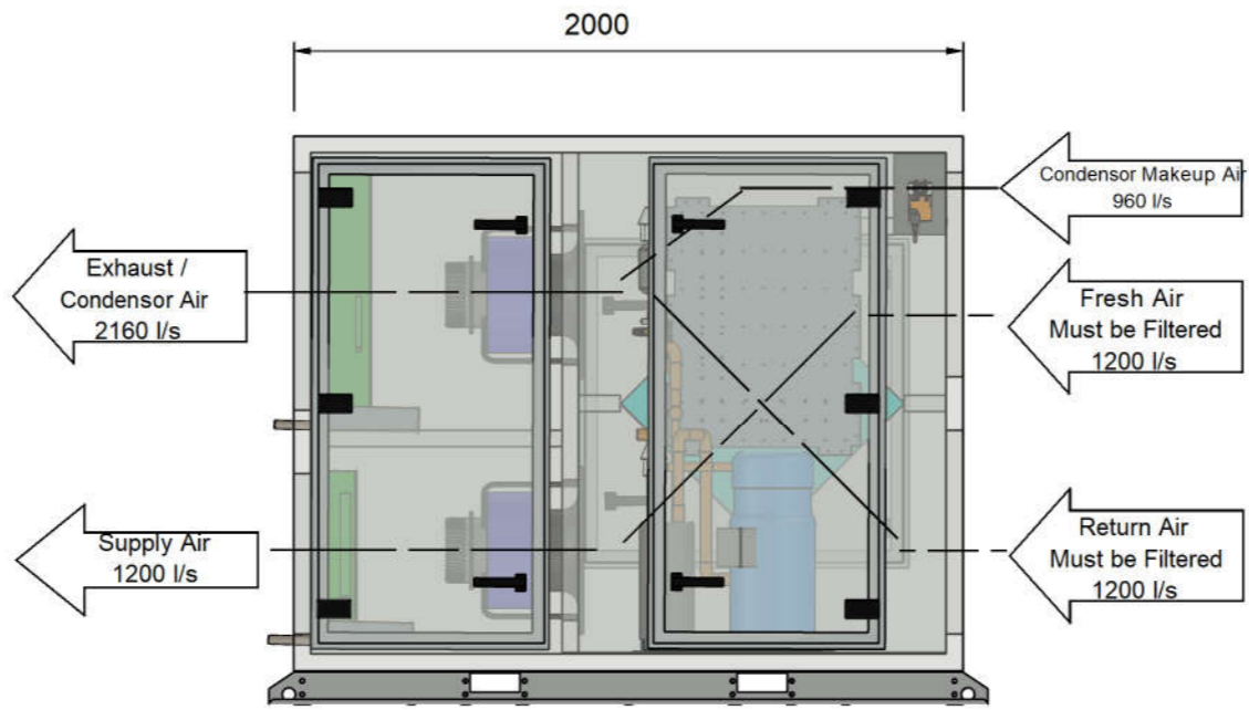
ELEVATION VIEW - COMPRESSOR ACCESS PANEL SIDE
