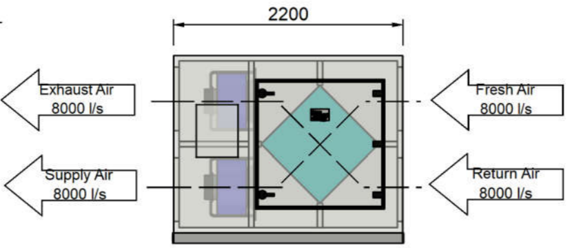
ELEVATION VIEW - ACCESS PANEL SIDE
