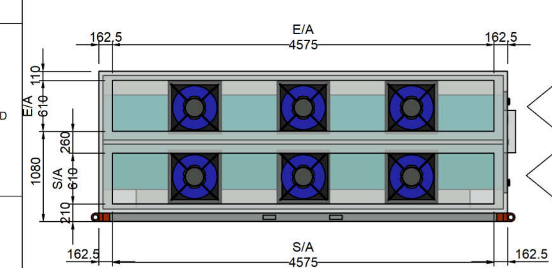
E/A & S/A SPIGOTS
