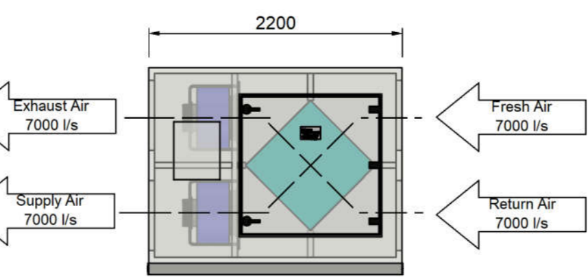
ELEVATION VIEW - ACCESS PANEL SIDE
