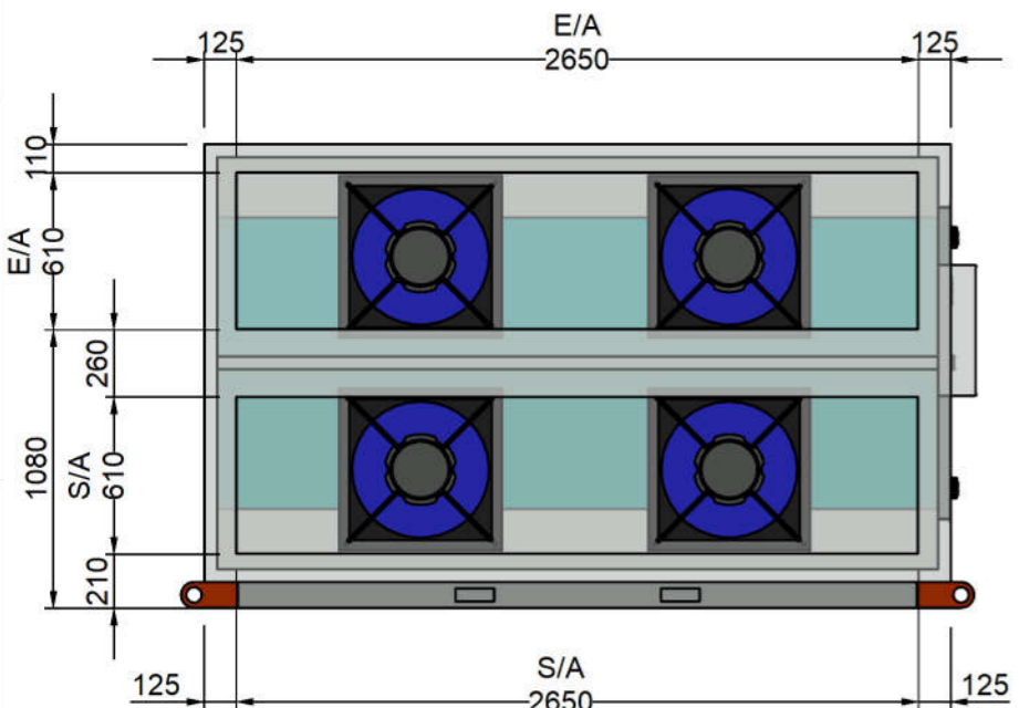
E/A & S/A SPIGOTS
