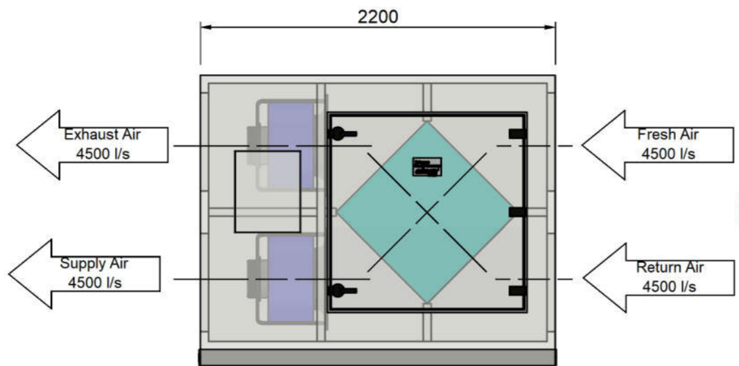
ELEVATION VIEW - ACCESS PANELS SIDE
