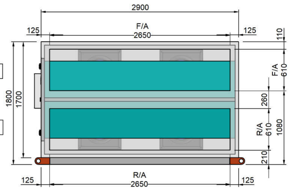
F/A & R/A SPIGOTS
