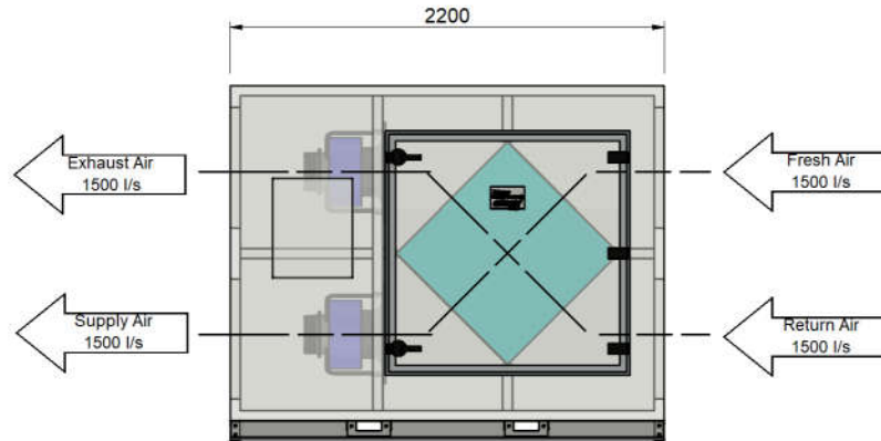
ELEVATION VIEW - ACCESS PANEL SIDE
