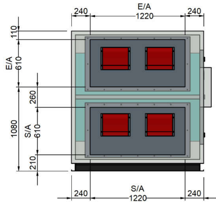
E/A & S/A SPIGOTS
