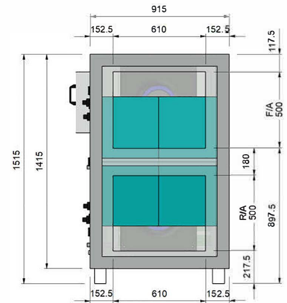
F/A & R/A SPIGOTS
