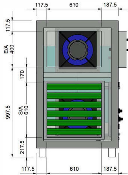
E/A & S/A SPIGOTS
