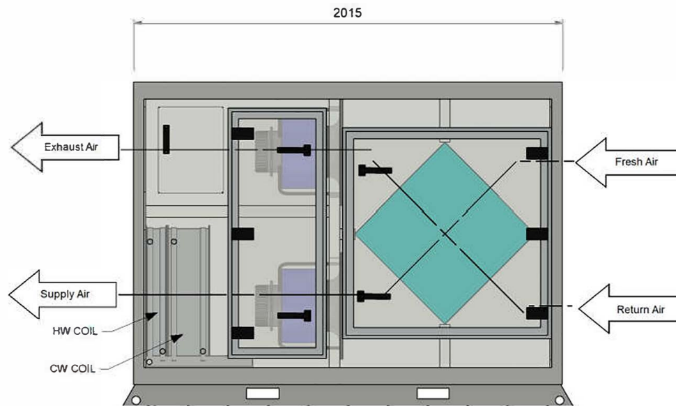
ELEVATION VIEW - ACCESS PANELS SIDE
