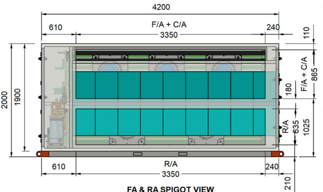
FA & RA SPIGOT VIEW
