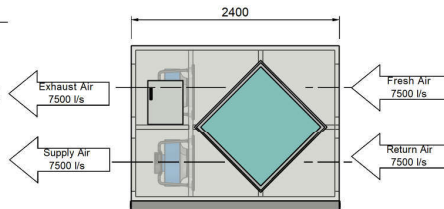
ELEVATION VIEW - ACCESS PANEL SIDE
