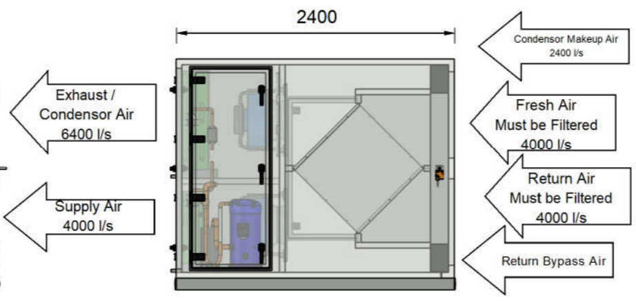
ELEVATION VIEW - COMPRESSOR ACCESS PANEL SIDE
