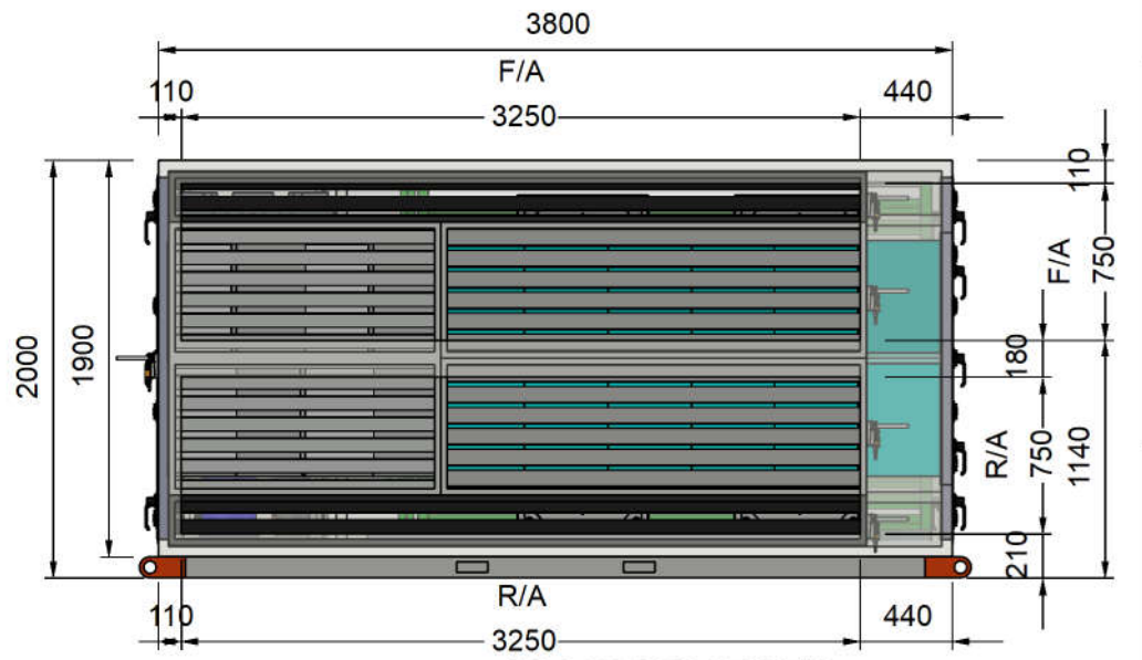
FA & RA SPIGOT VIEW
