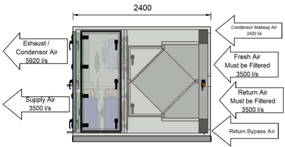
ELEVATION VIEW - ACCESS PANELS SIDE
