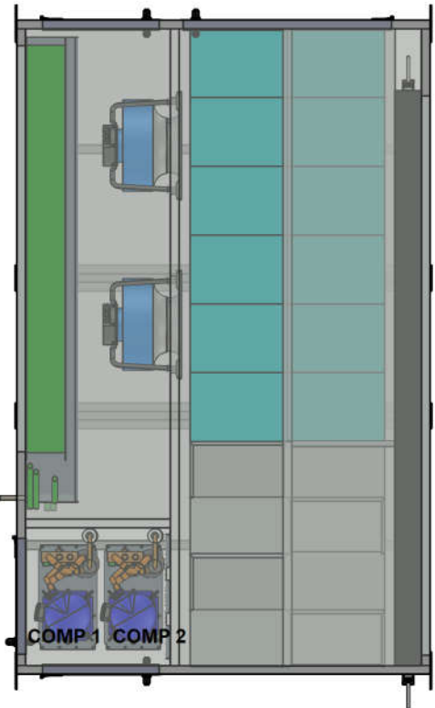
PLAN VIEW
