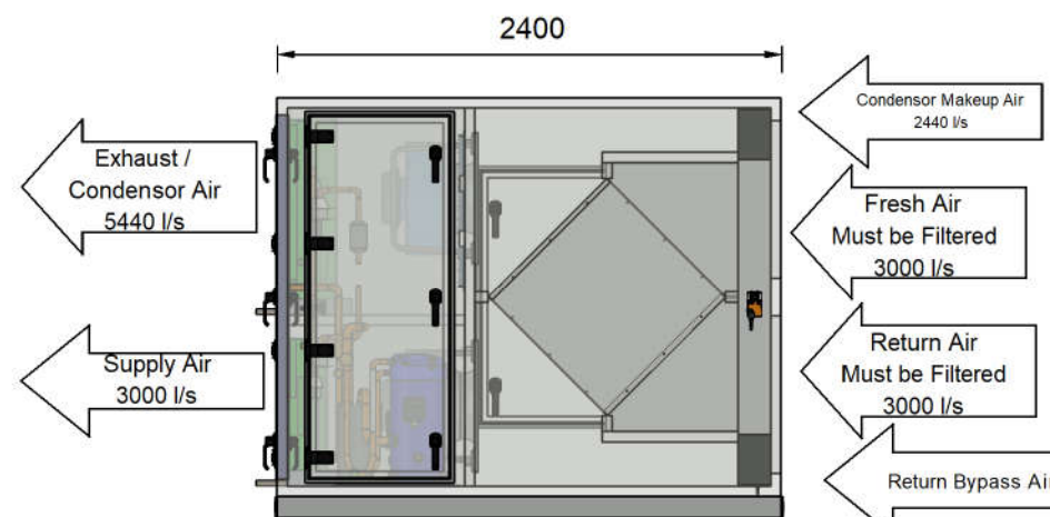
ELEVATION VIEW - ACCESS PANELS SIDE
