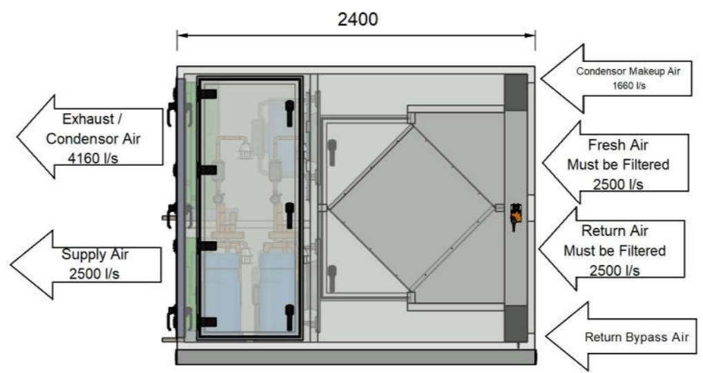
ELEVATION VIEW - ACCESS PANELS SIDE
