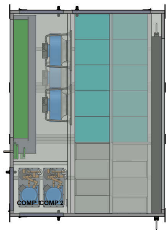
PLAN VIEW
