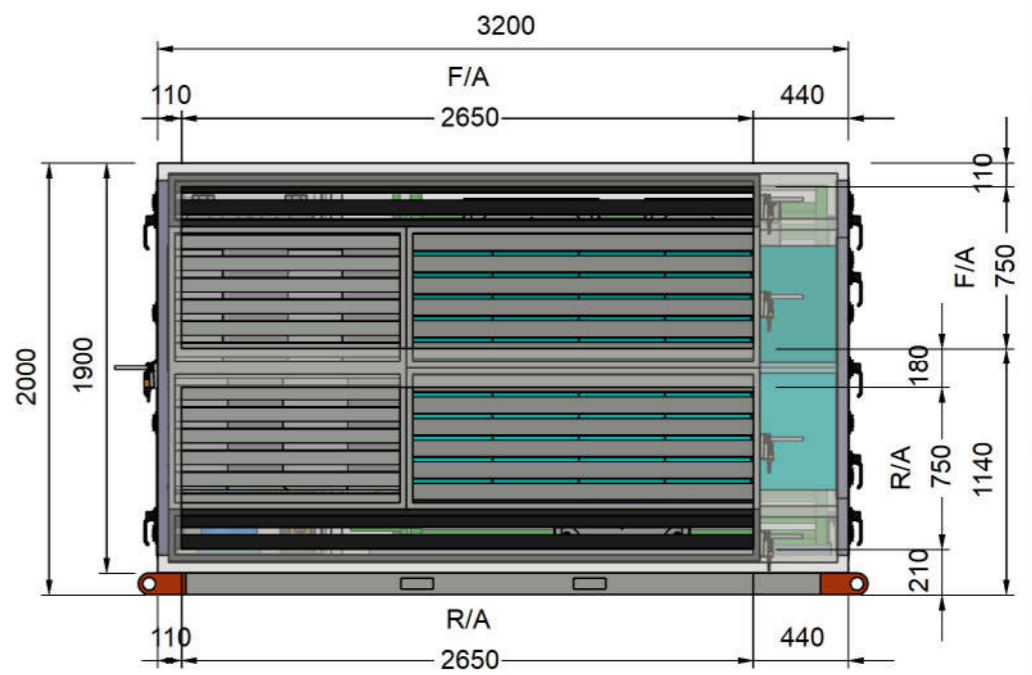
FA & RA SPIGOT VIEW
