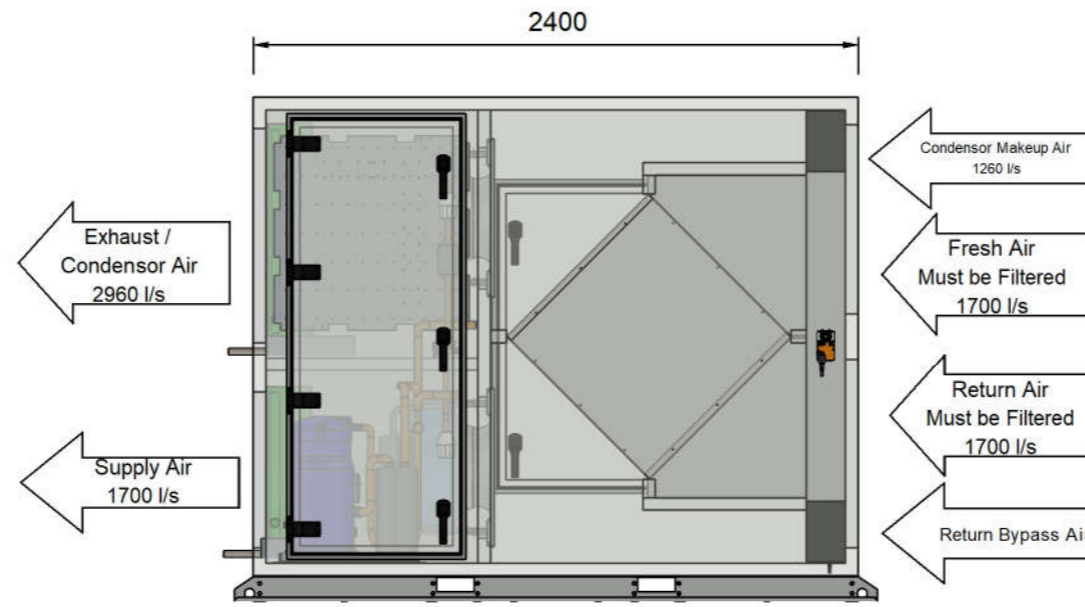
ELEVATION VIEW - ACCESS PANELS SIDE
