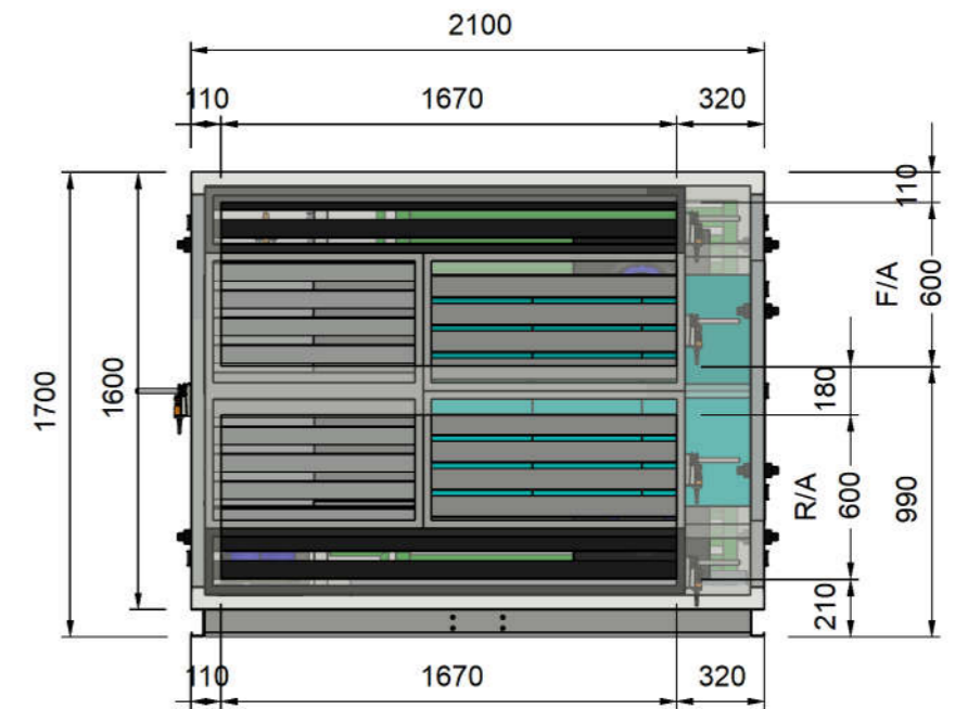
FA & RA SPIGOT VIEW
